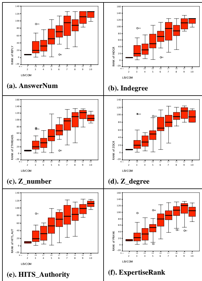
Figure 7: Box plots of algorithm rankings vs. human ratings
