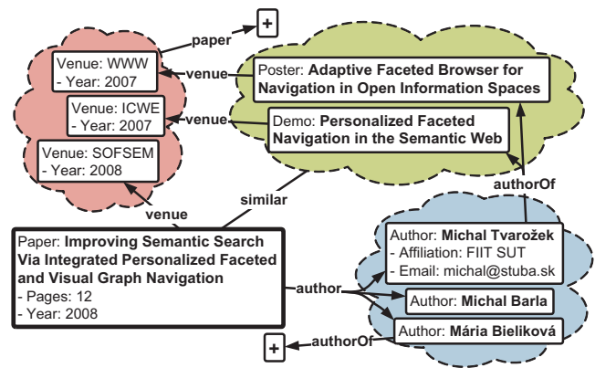
Figure 2: Graphical instance attribute visualization.
